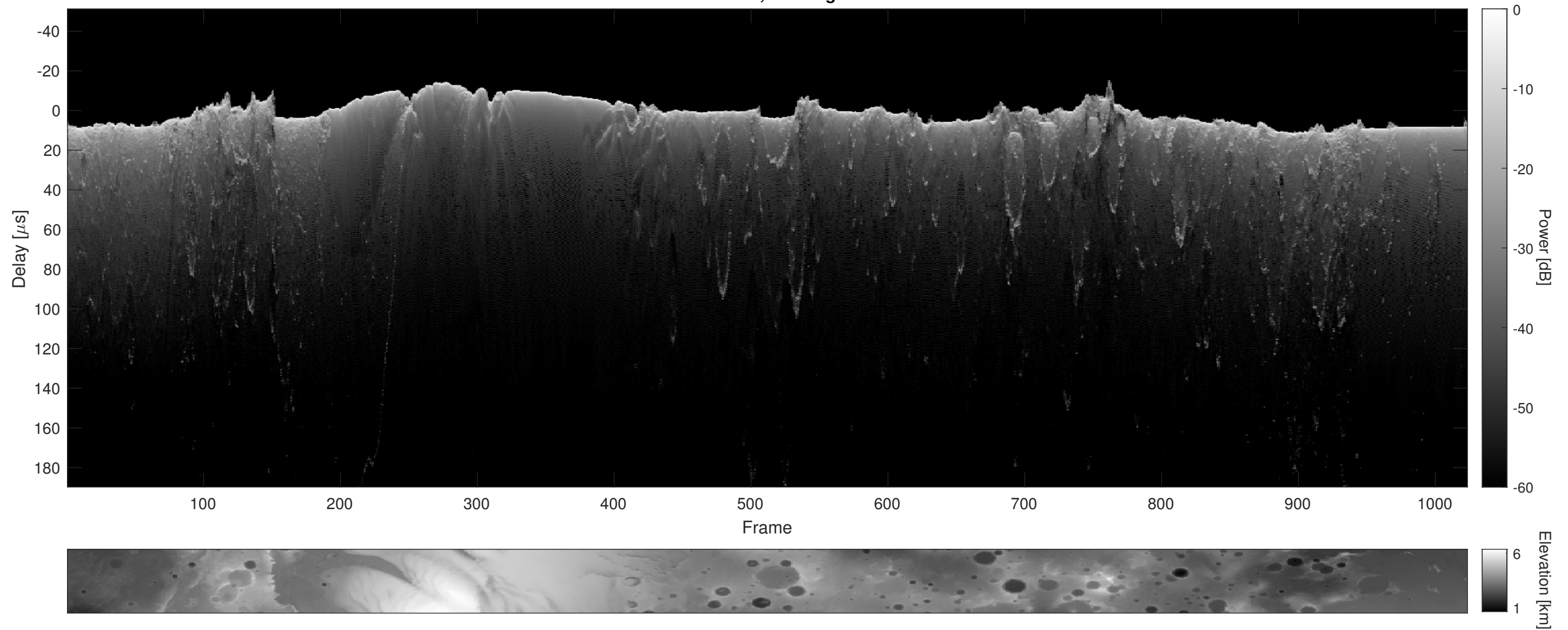
Orbit 10684, Cluttergram
