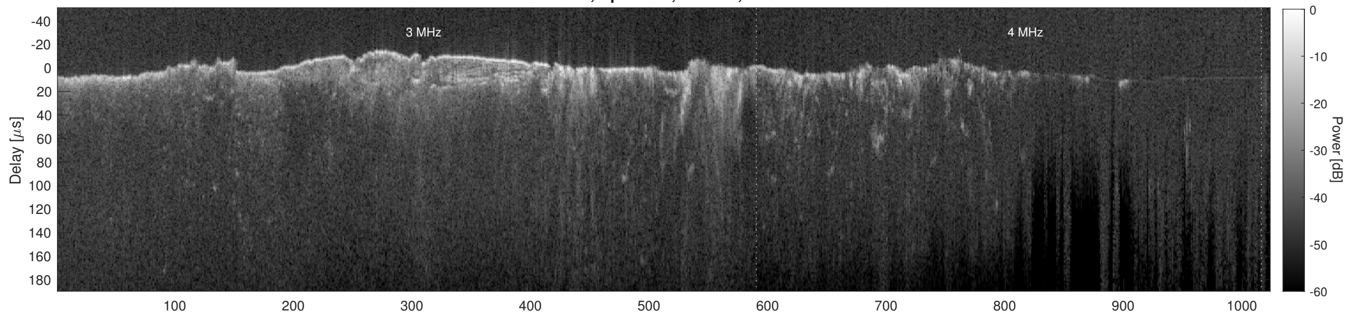
Orbit 10684, Cluttergram
