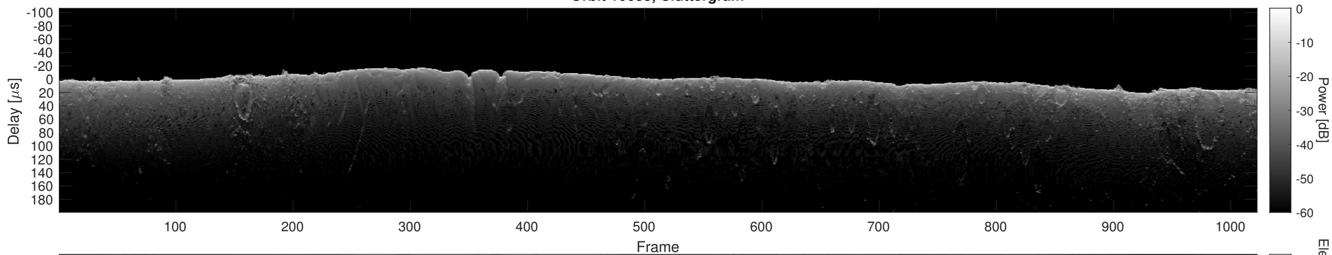
Orbit 10688, Cluttergram
