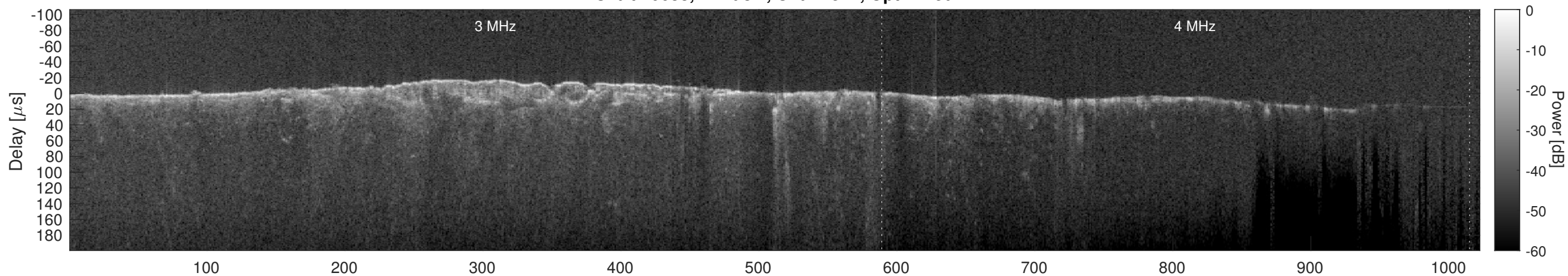
Orbit 10688, Cluttergram
