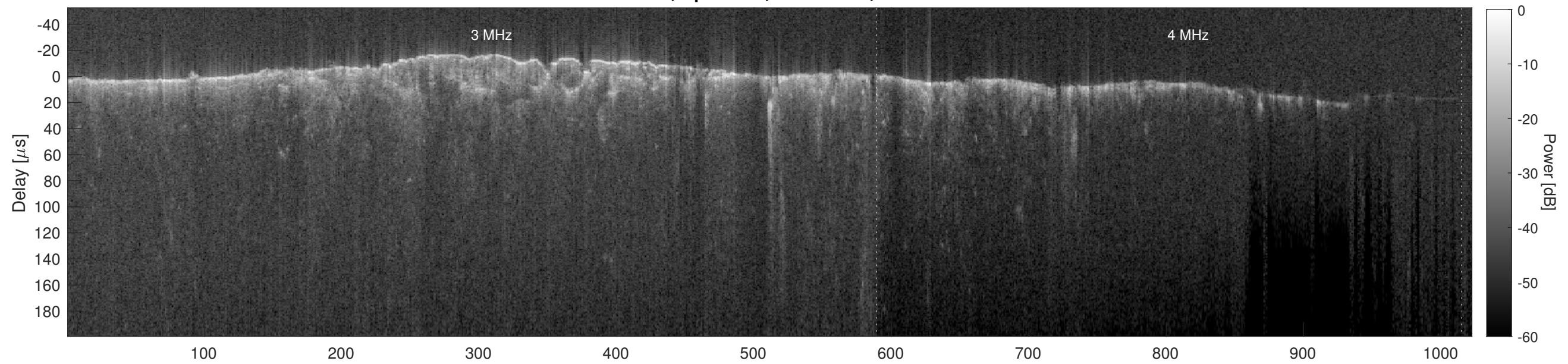
Orbit 10688, Cluttergram
