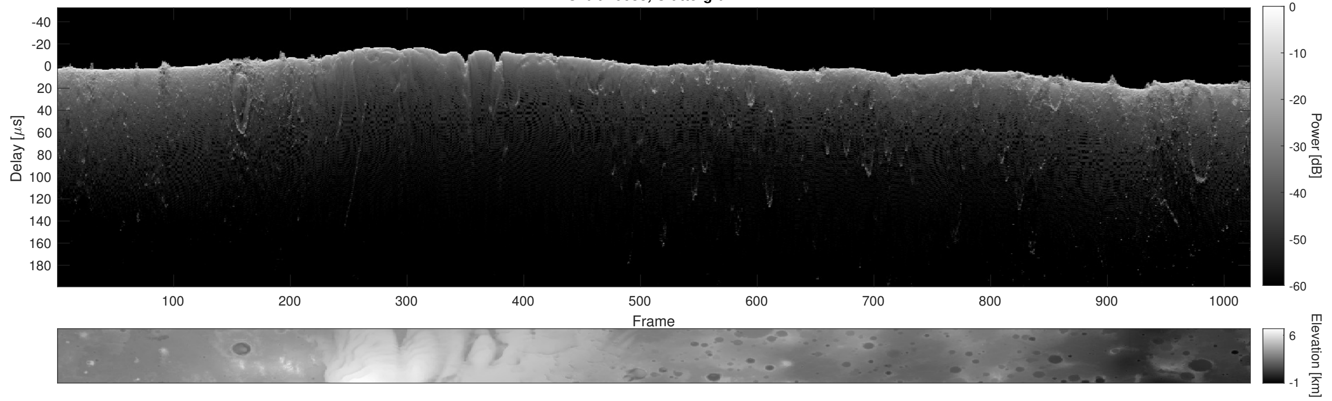
Orbit 10688, Cluttergram
