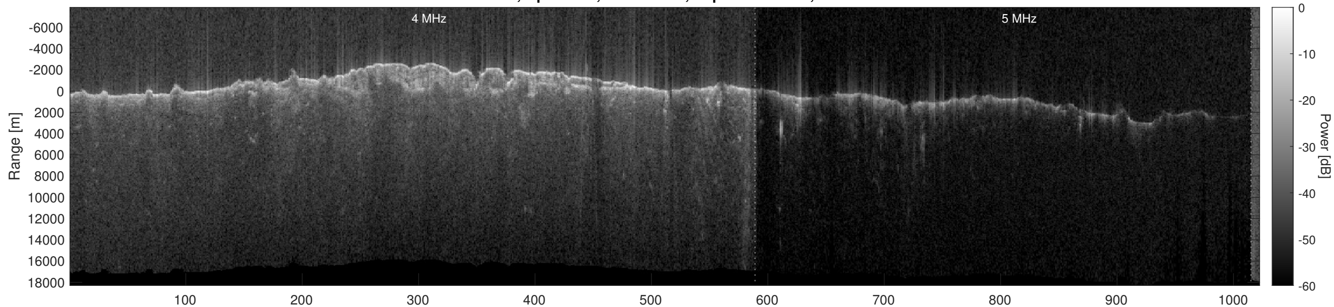
Orbit 10688, Optimized, No Window, Depth-Corrected, Channel 2
