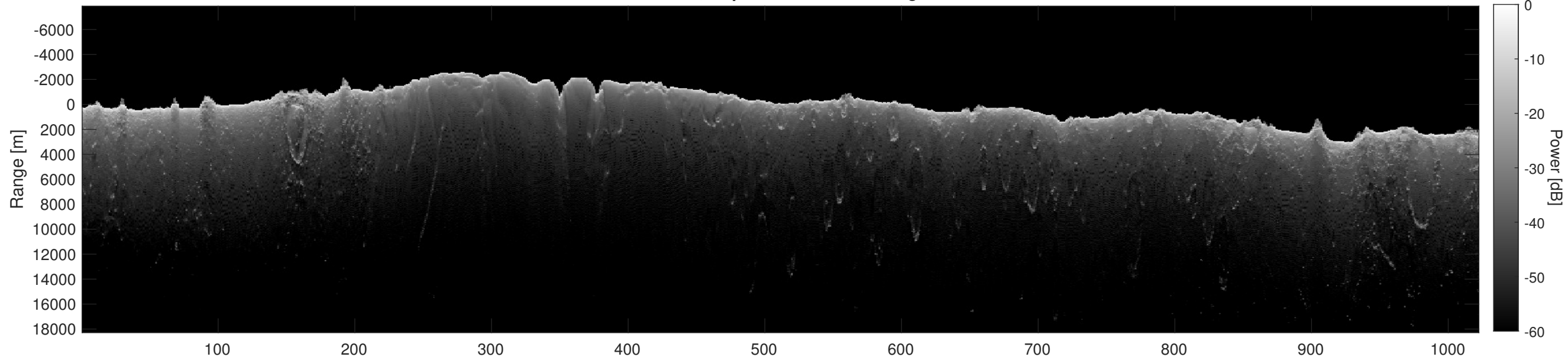
Orbit 10688, Depth-Corrected Cluttergram
