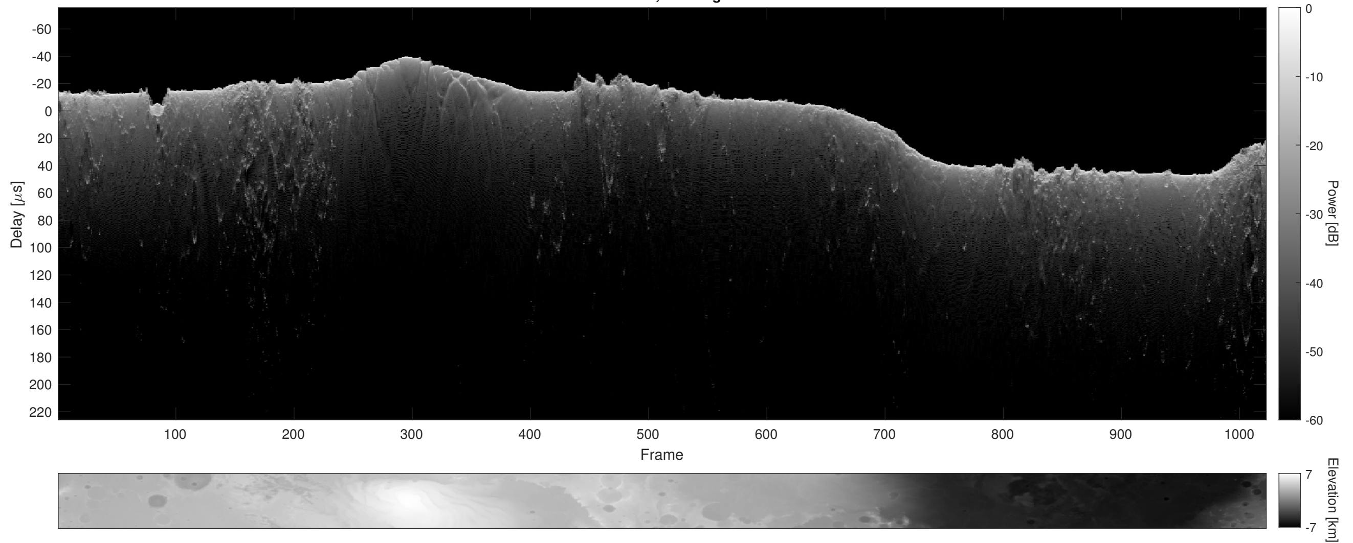
Orbit 10689, Cluttergram
