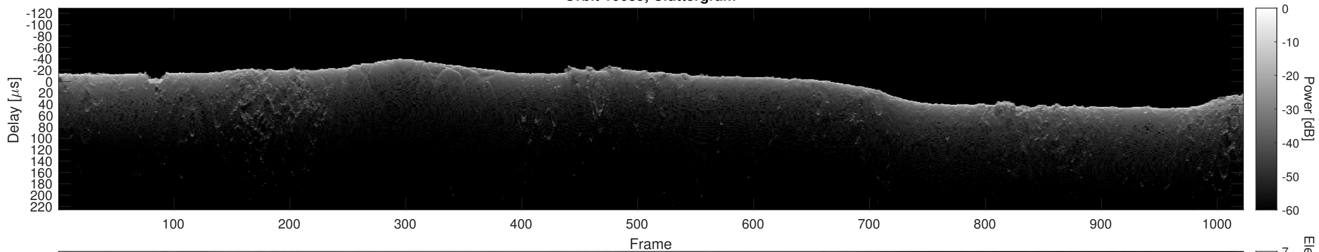
Orbit 10689, Cluttergram
