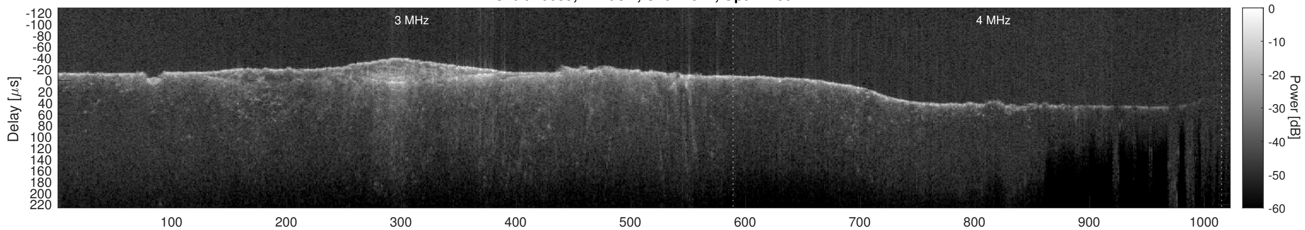
Orbit 10689, Cluttergram
