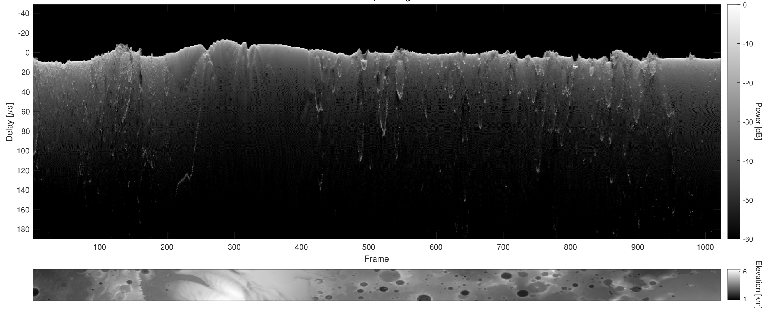
Orbit 10691, Cluttergram
