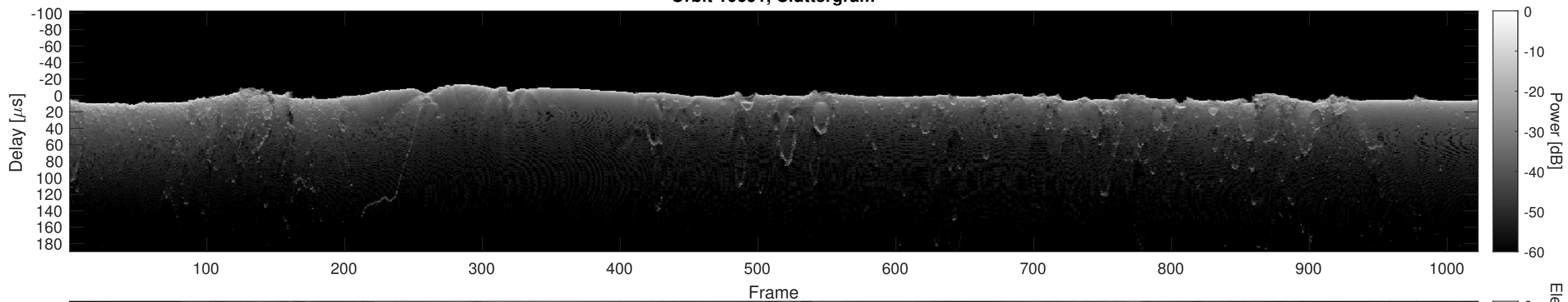
Orbit 10691, Cluttergram
