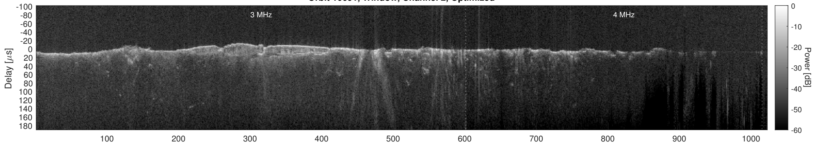
Orbit 10691, Cluttergram
