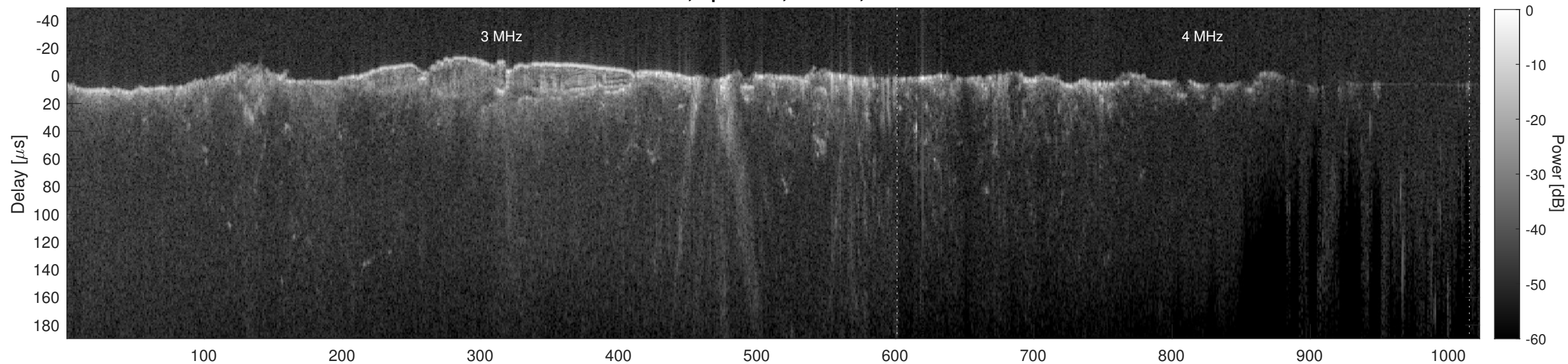
Orbit 10691, Cluttergram
