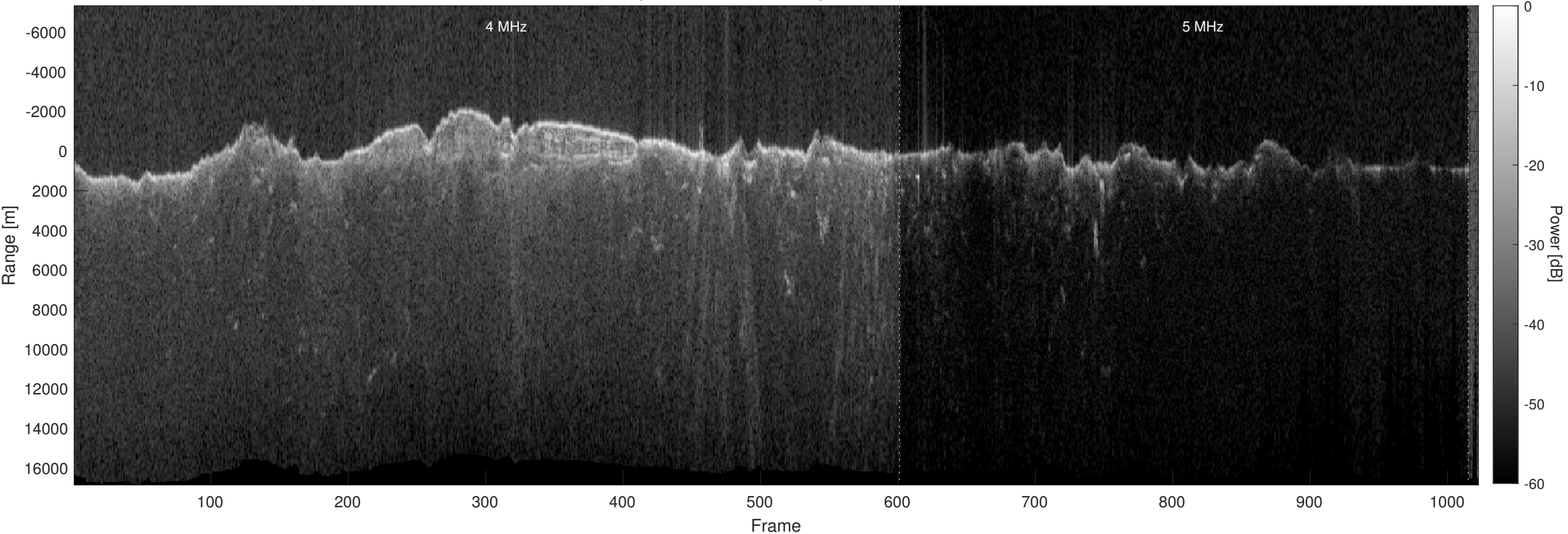
Orbit 10691, Optimized, Window, Depth-Corrected, Channel 2
