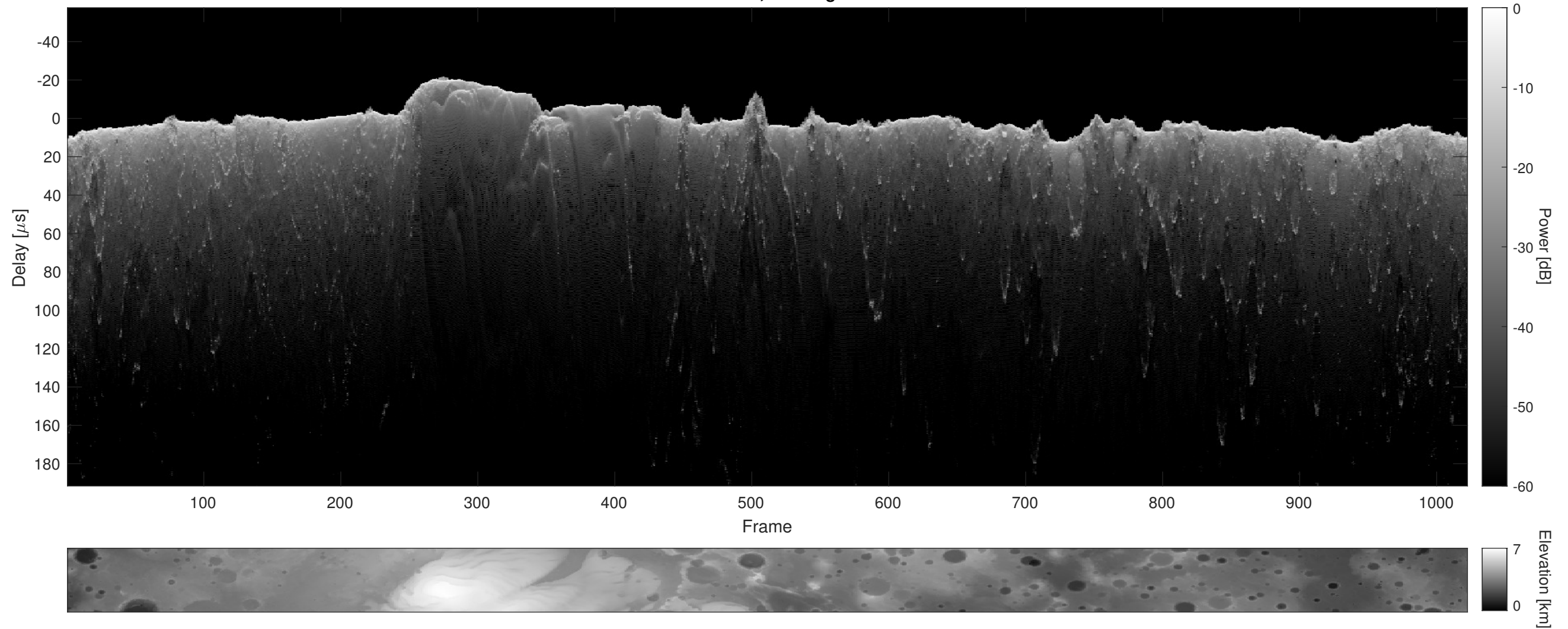
Orbit 10692, Cluttergram
