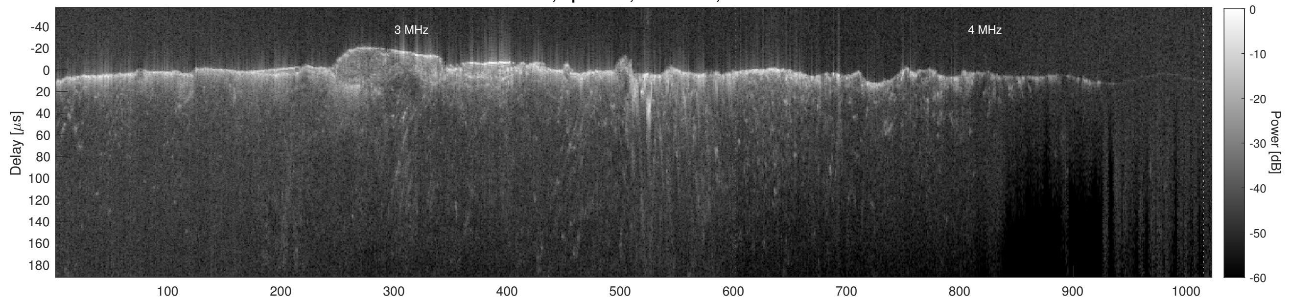
Orbit 10692, Cluttergram
