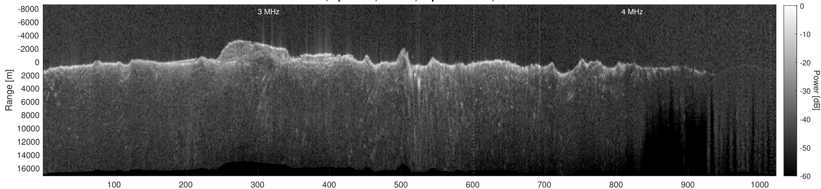
Orbit 10692, Depth-Corrected Cluttergram
