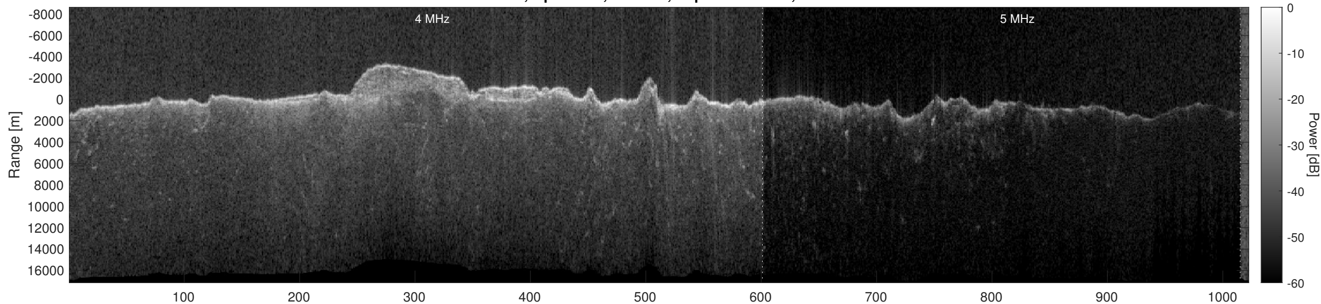
Orbit 10692, Optimized, Window, Depth-Corrected, Channel 2
