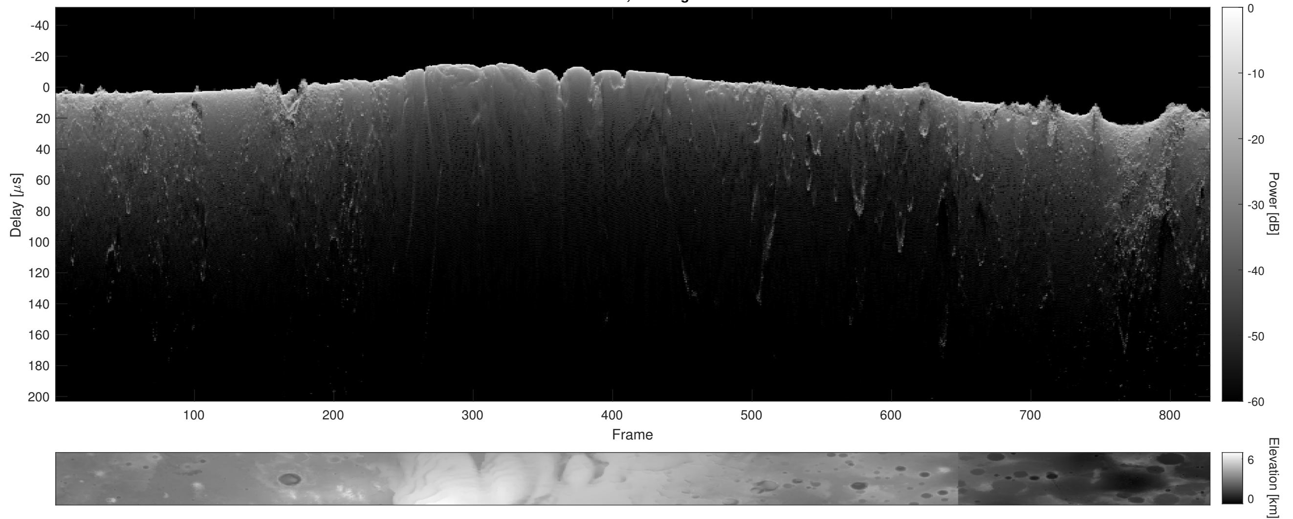
Orbit 10695, Cluttergram
