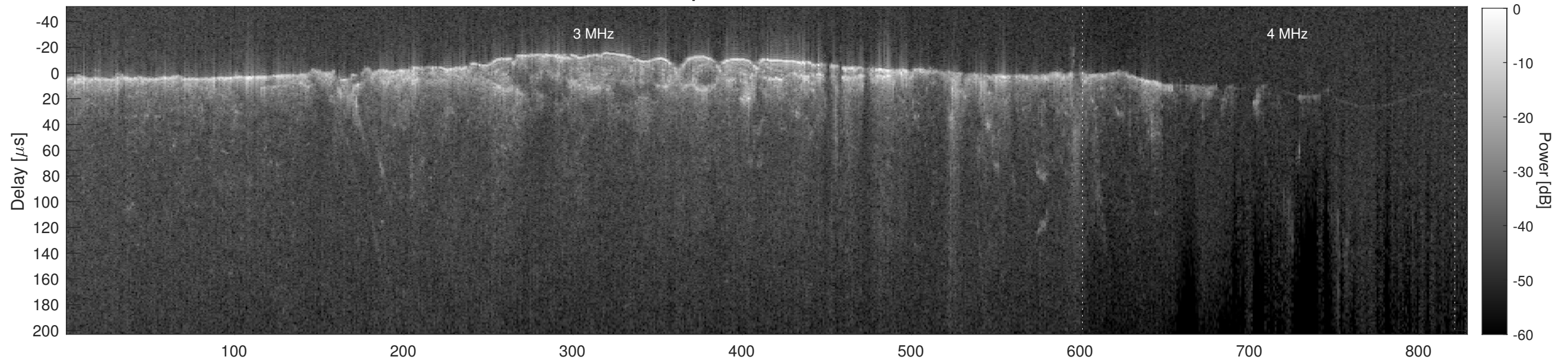
Orbit 10695, Cluttergram
