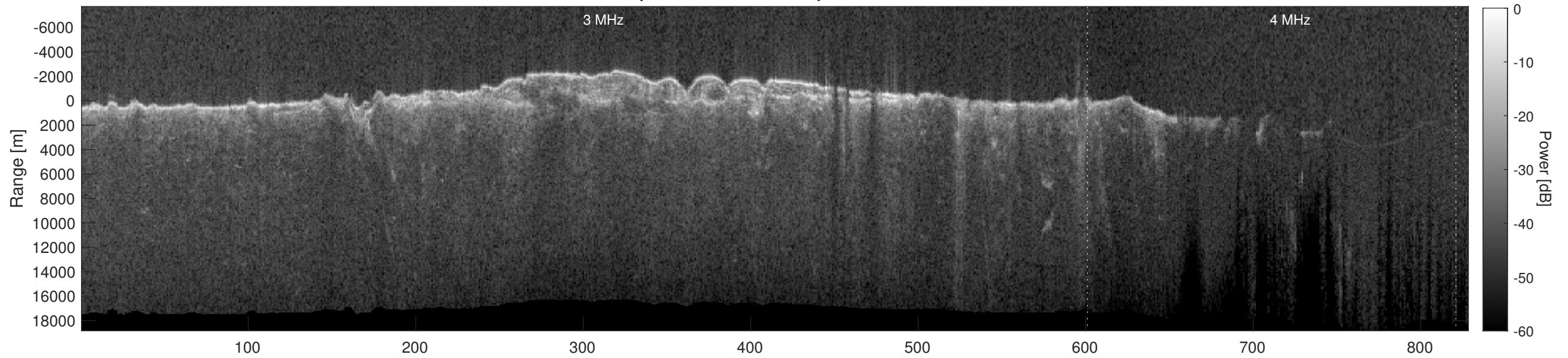
Orbit 10695, Depth-Corrected Cluttergram
