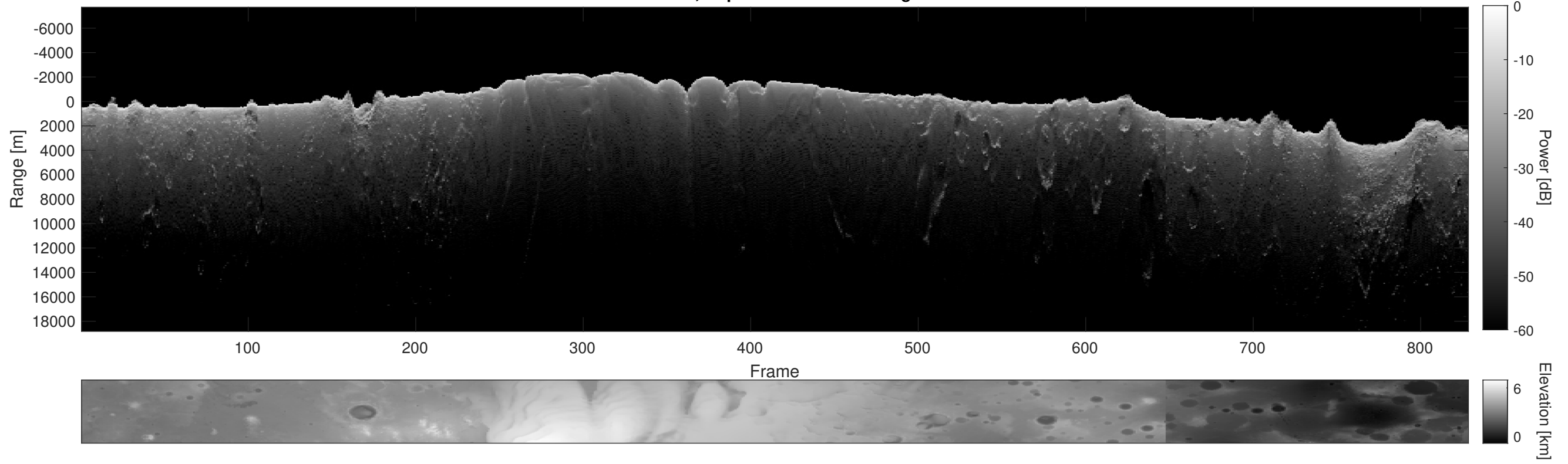
Orbit 10695, Depth-Corrected Cluttergram
