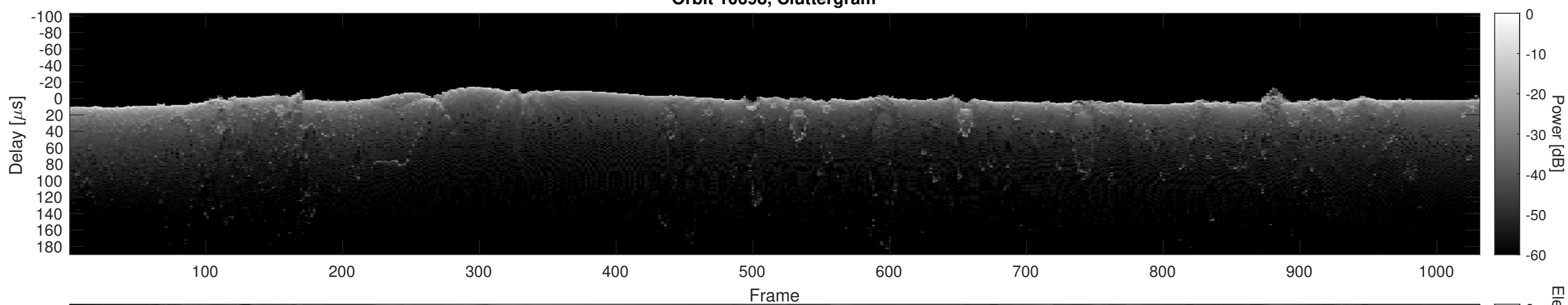
Orbit 10698, Cluttergram
