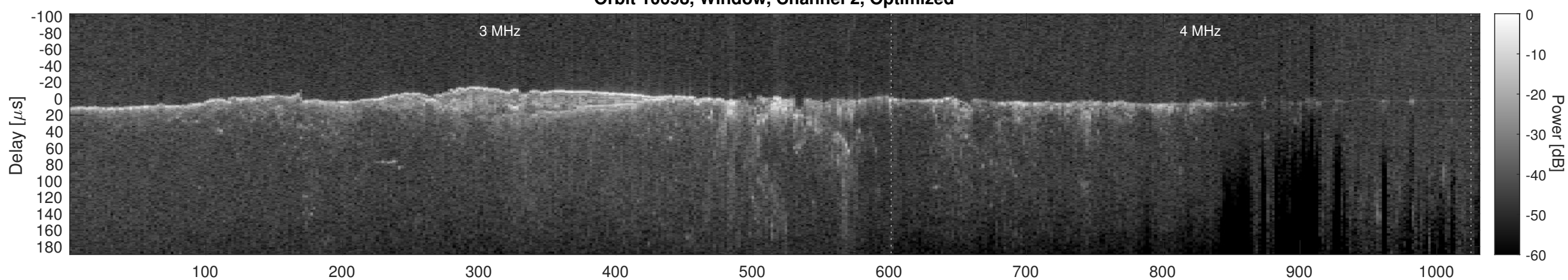
Orbit 10698, Cluttergram
