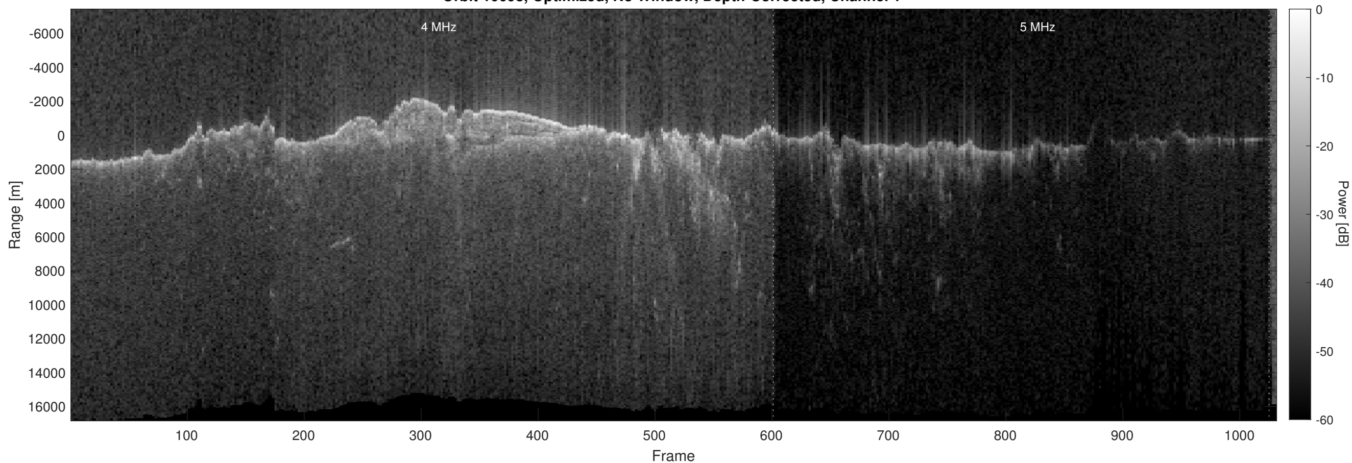
Orbit 10698, Optimized, No Window, Depth-Corrected, Channel 2
