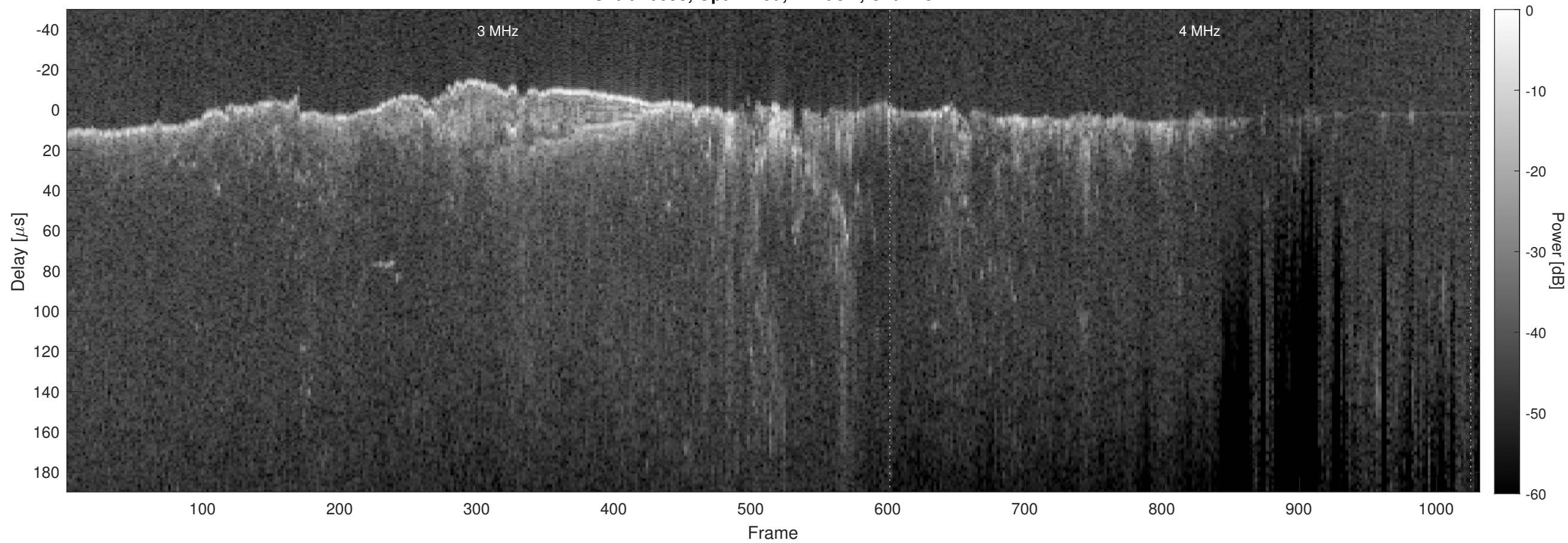
Orbit 10698, Optimized, Window, Channel 2
