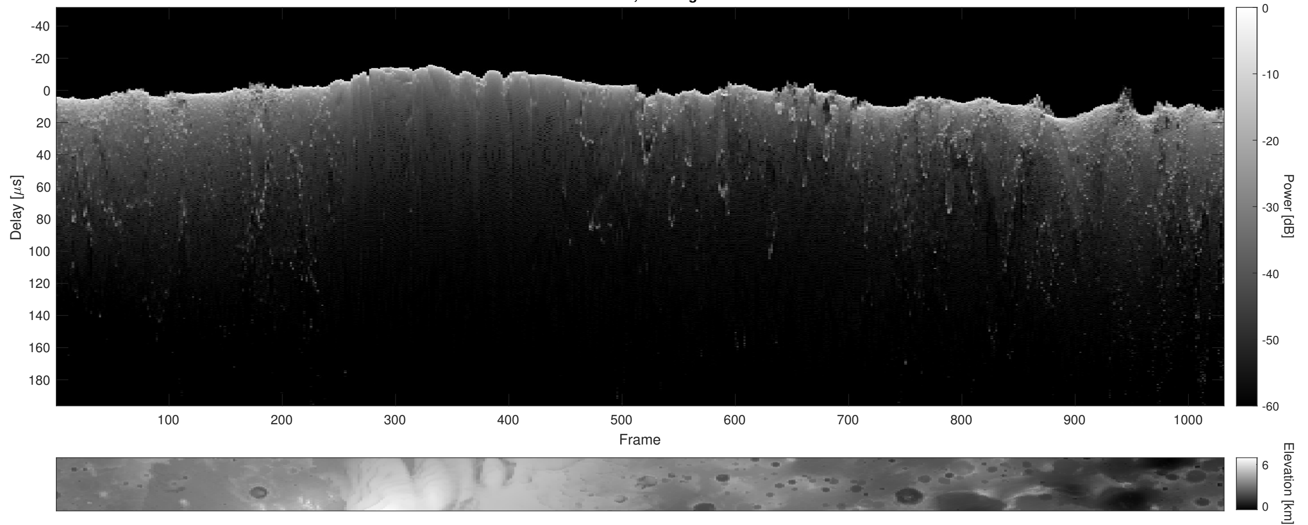
Orbit 10702, Cluttergram
