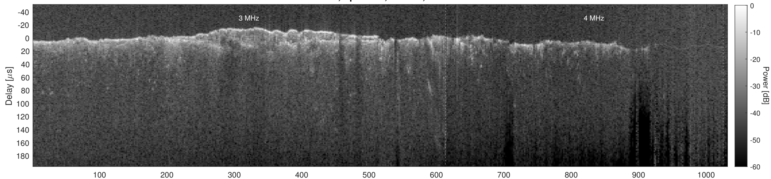
Orbit 10702, Cluttergram
