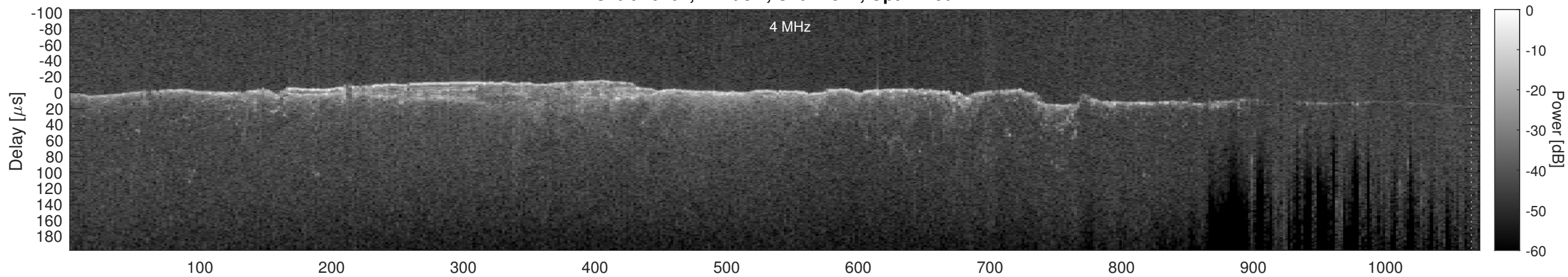
Orbit 10704, Cluttergram
