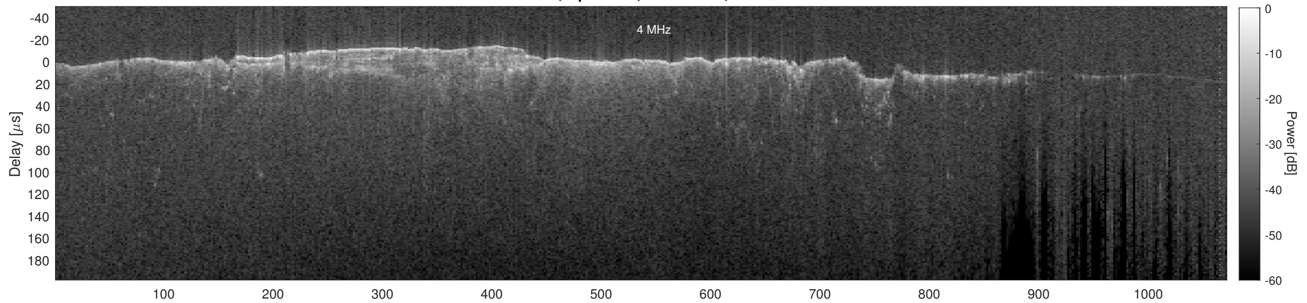
Orbit 10704, Cluttergram
