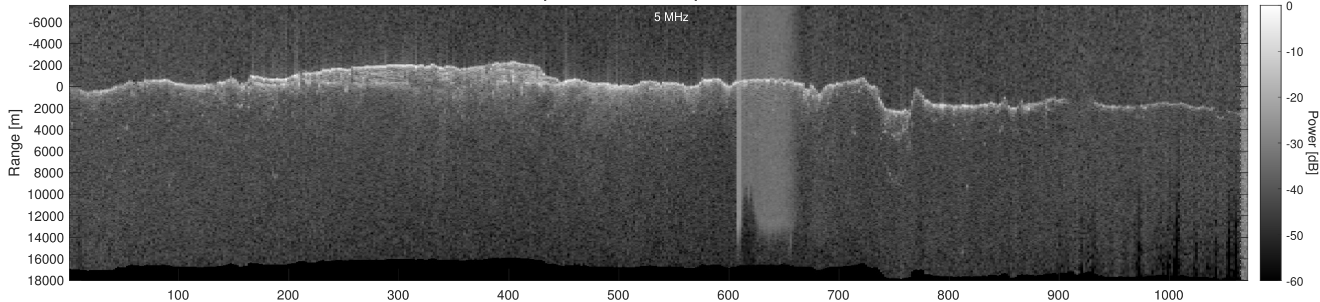
Orbit 10704, Optimized, Window, Depth-Corrected, Channel 2
