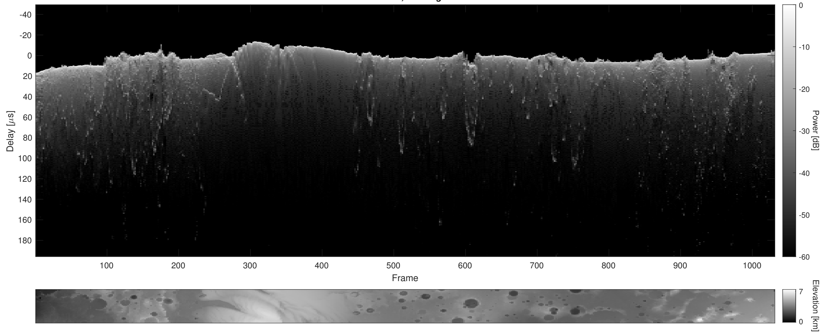
Orbit 10705, Cluttergram
