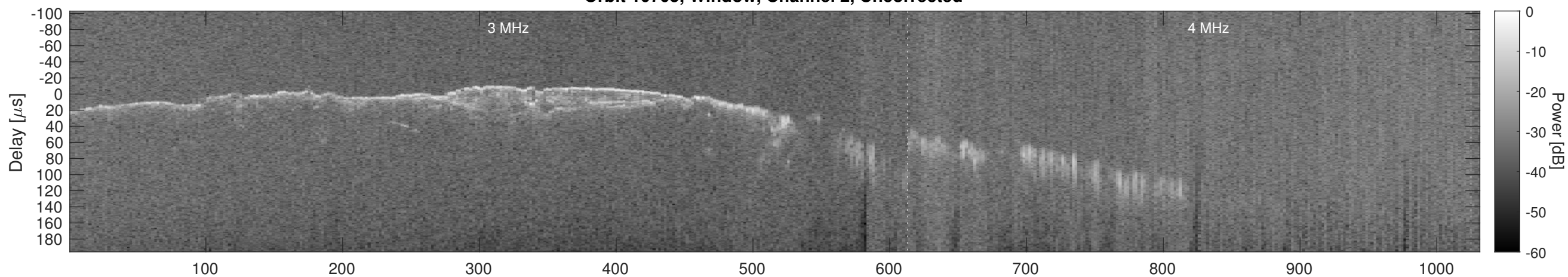
Orbit 10705, Window, Channel 2, Chapman
