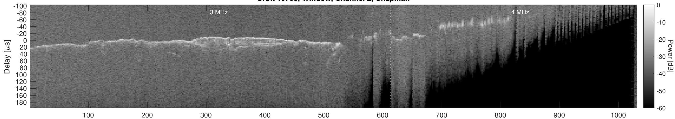
Orbit 10705, Window, Channel 2, Optimized
