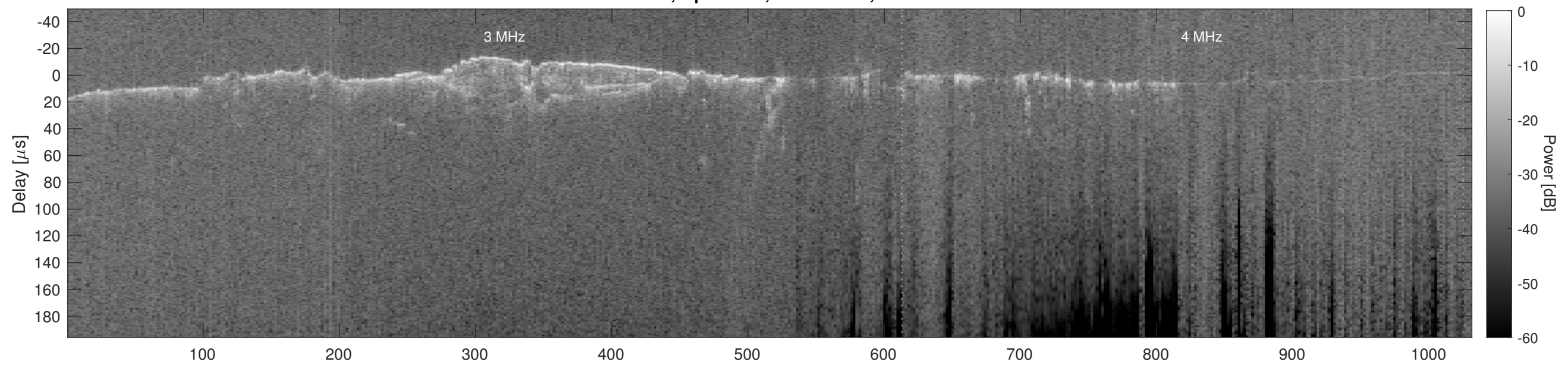
Orbit 10705, Cluttergram
