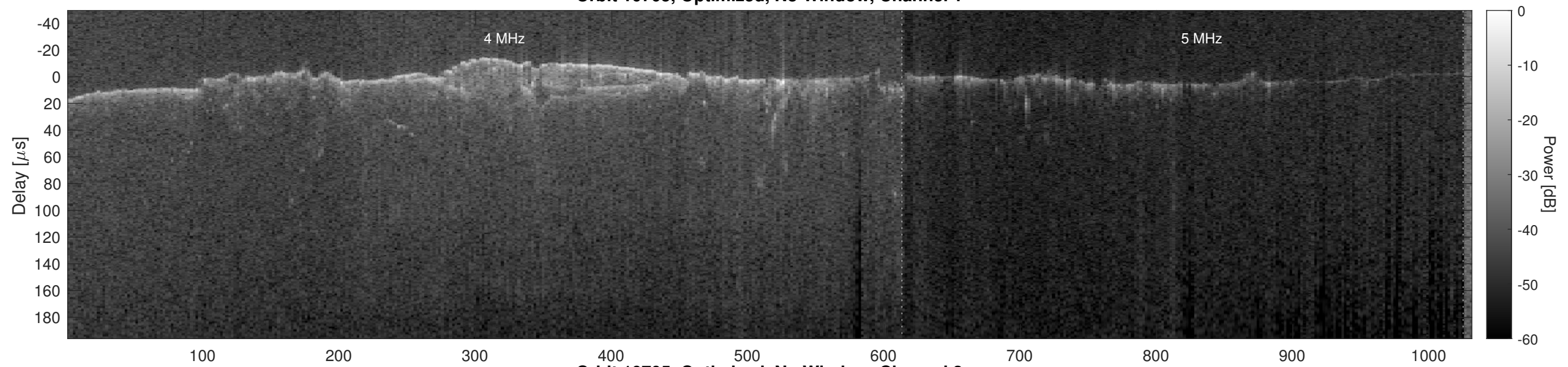
Orbit 10705, Optimized, No Window, Channel 2
