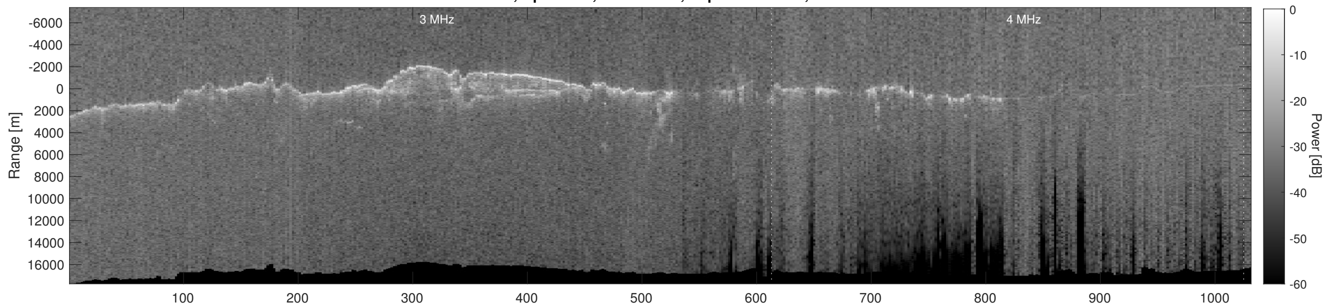
Orbit 10705, Depth-Corrected Cluttergram
