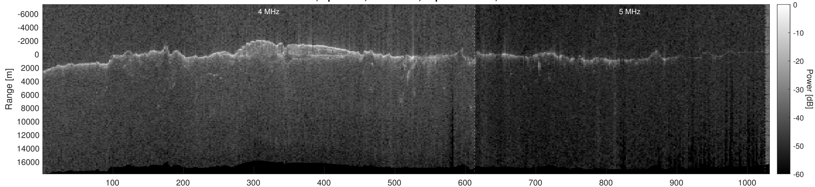
Orbit 10705, Optimized, No Window, Depth-Corrected, Channel 2
