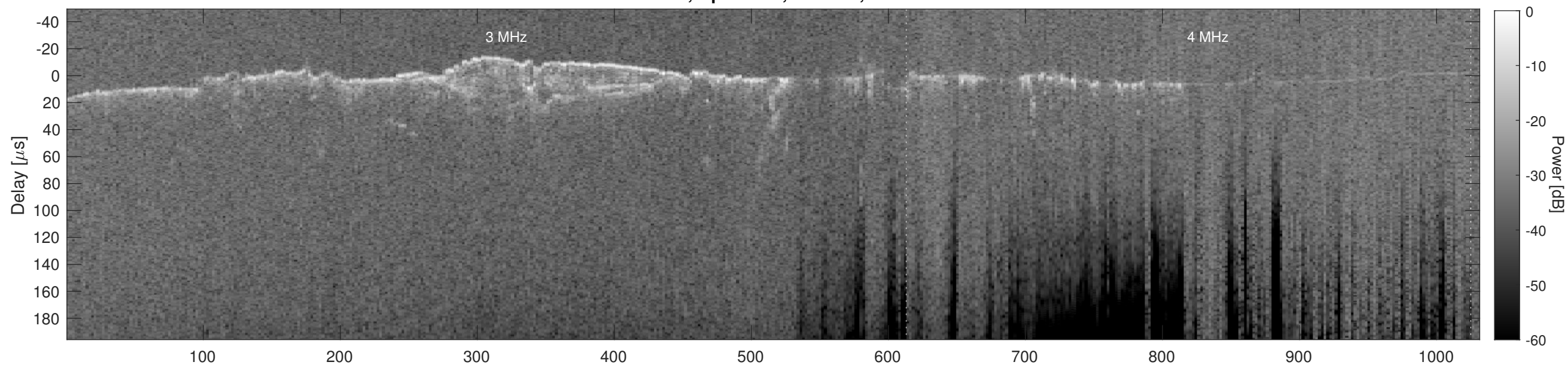
Orbit 10705, Cluttergram
