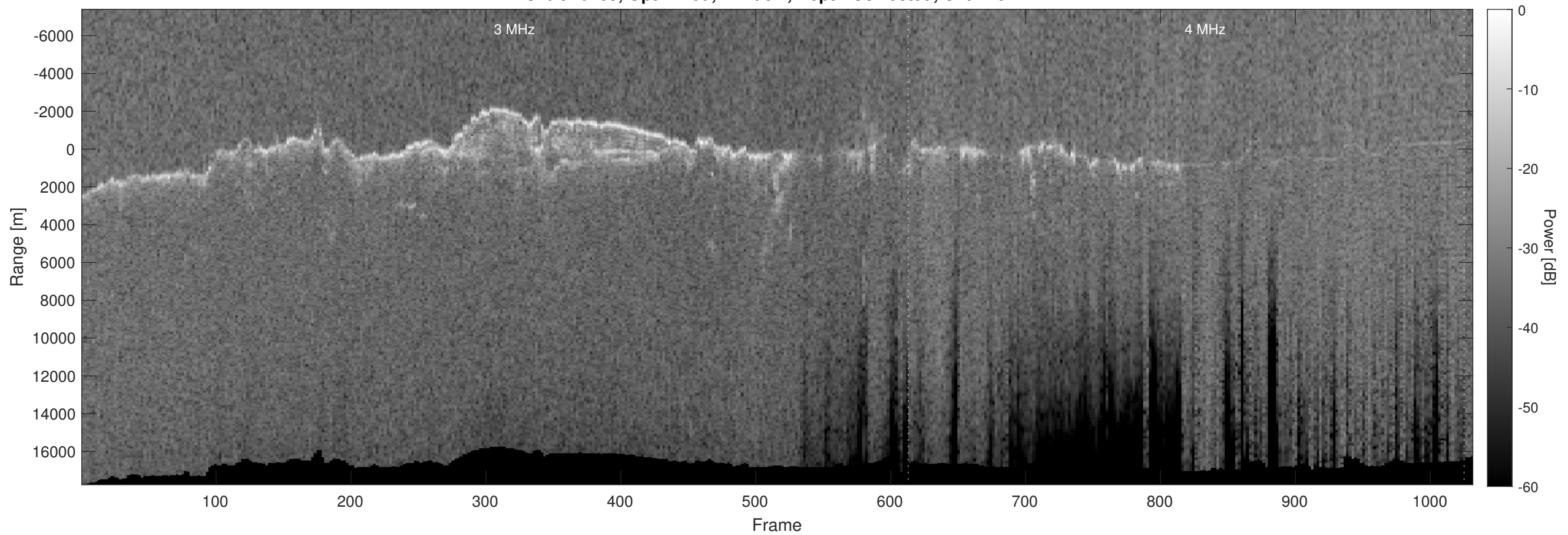
Orbit 10705, Optimized, Window, Depth-Corrected, Channel 2
