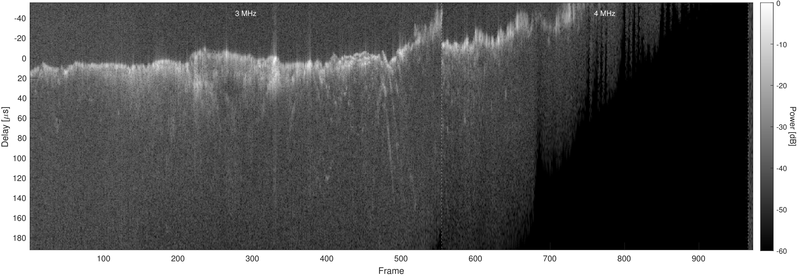
Orbit 10706, Chapman, No Window, Channel 2
