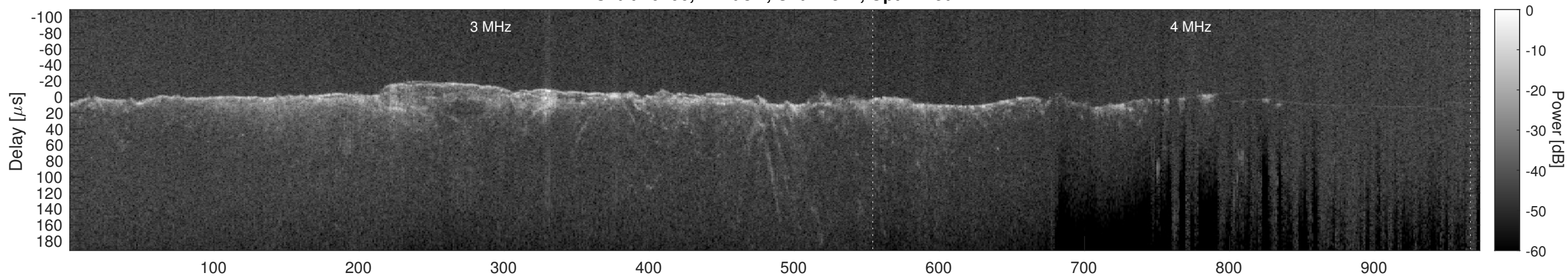
Orbit 10706, Cluttergram
