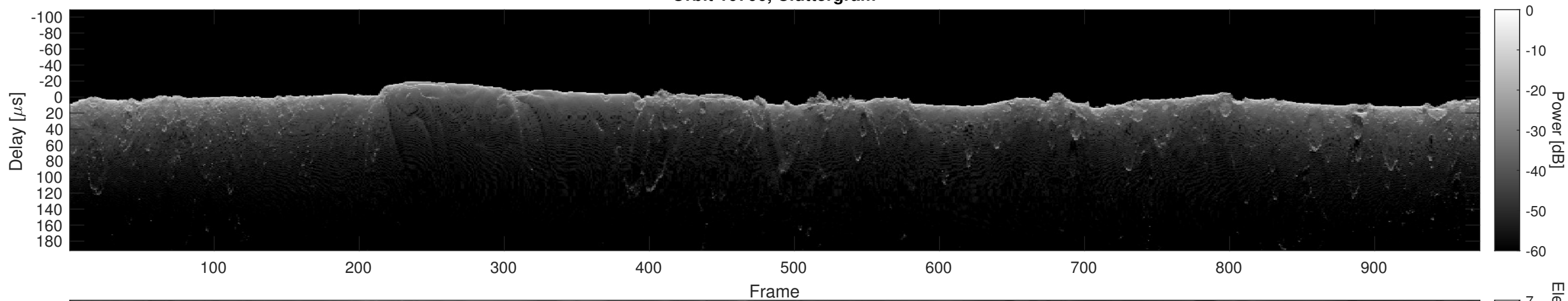
Orbit 10706, Cluttergram
