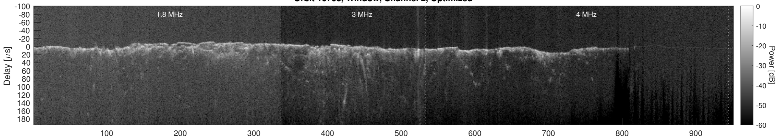
Orbit 10708, Cluttergram
