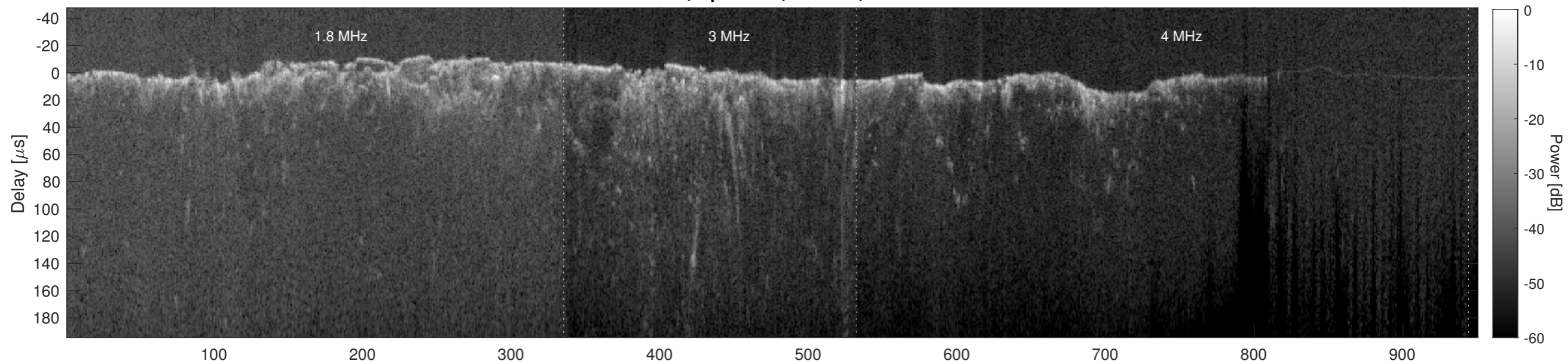
Orbit 10708, Cluttergram
