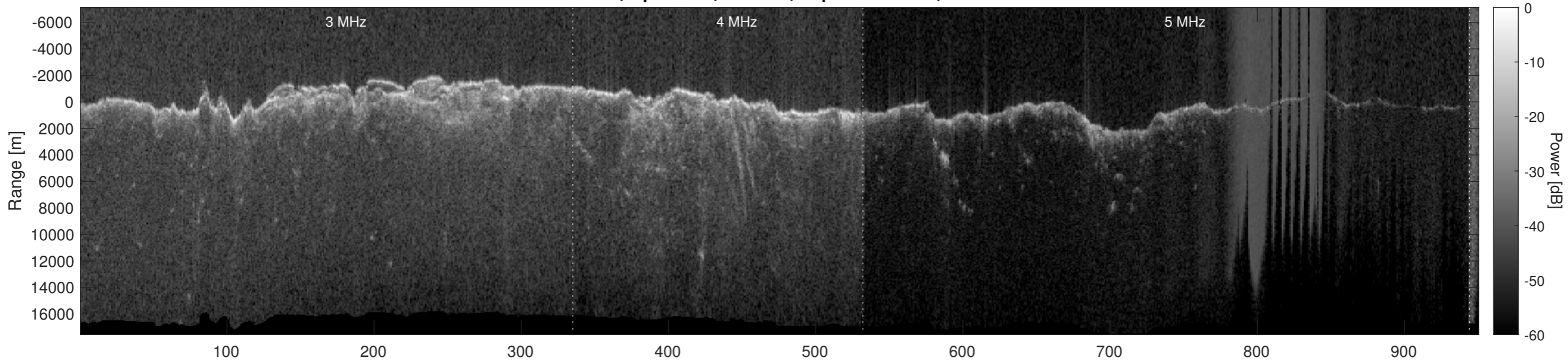
Orbit 10708, Optimized, Window, Depth-Corrected, Channel 2
