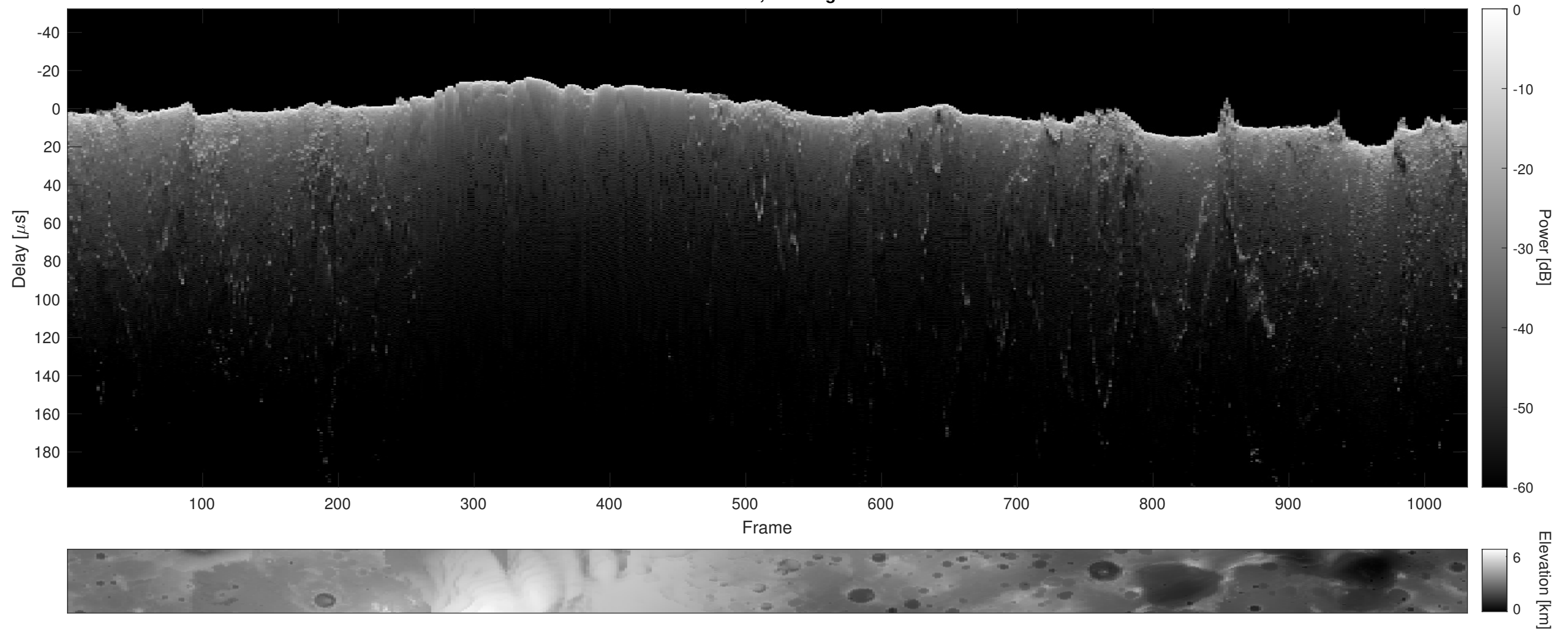
Orbit 10709, Cluttergram
