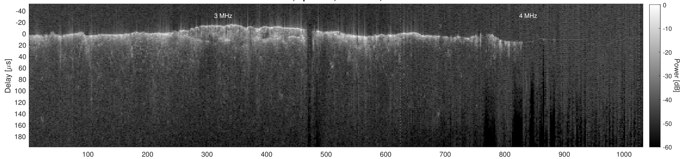
Orbit 10709, Cluttergram
