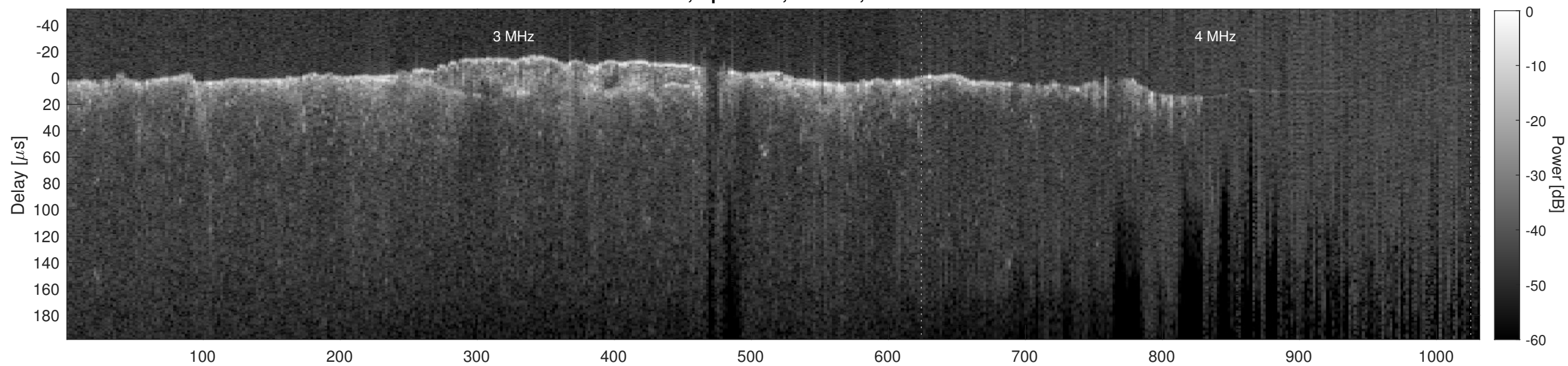
Orbit 10709, Cluttergram
