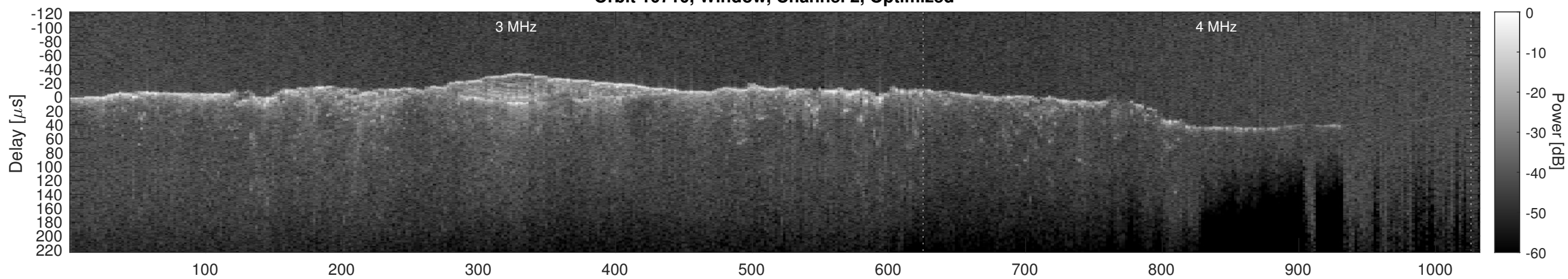
Orbit 10710, Cluttergram
