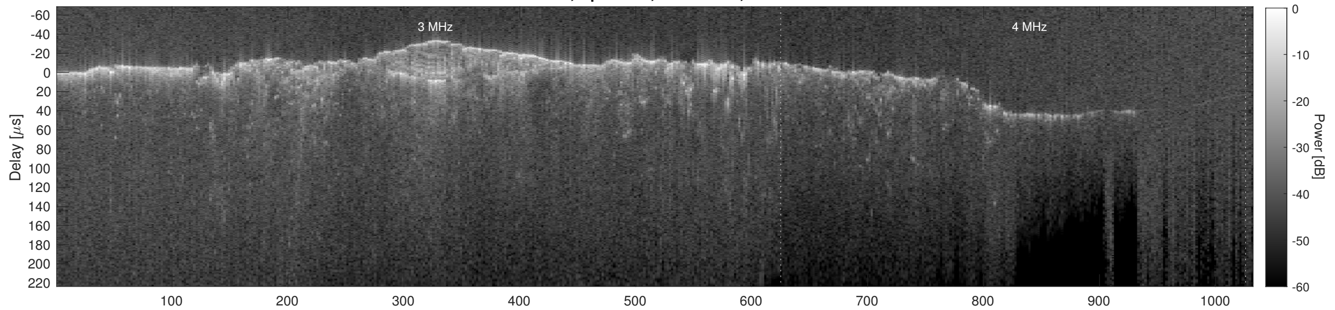
Orbit 10710, Cluttergram
