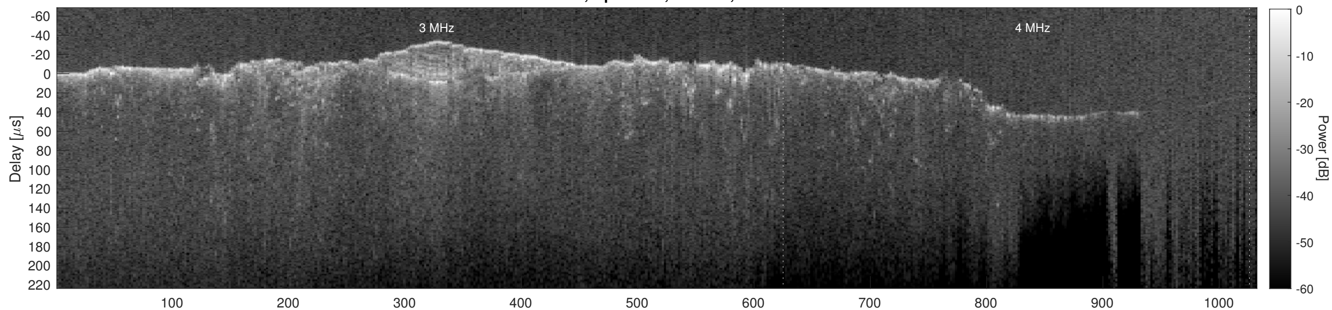
Orbit 10710, Cluttergram
