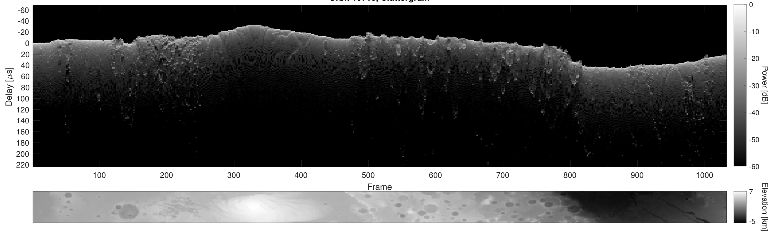
Orbit 10710, Cluttergram
