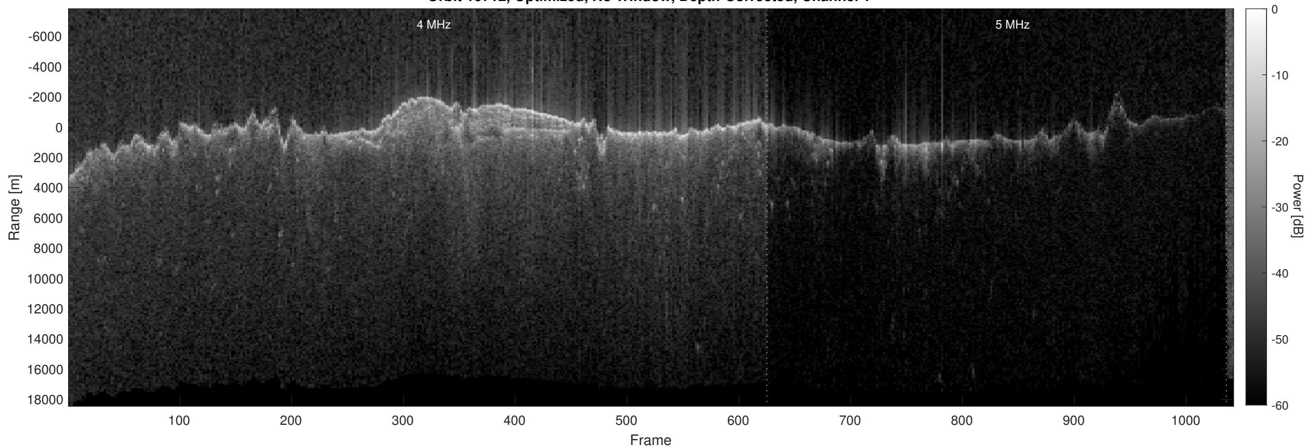
Orbit 10712, Optimized, No Window, Depth-Corrected, Channel 2
