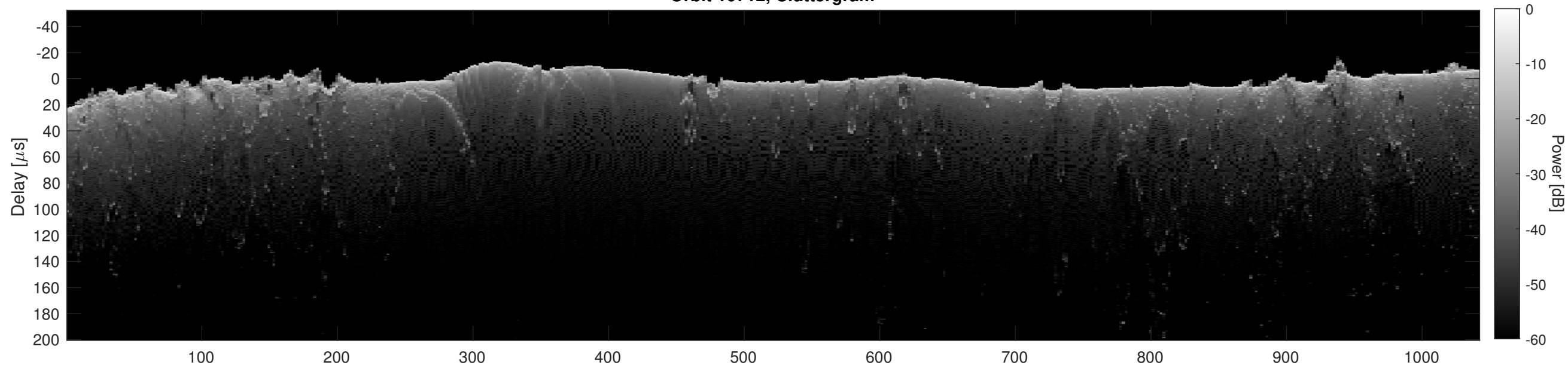
Orbit 10712, Cluttergram
