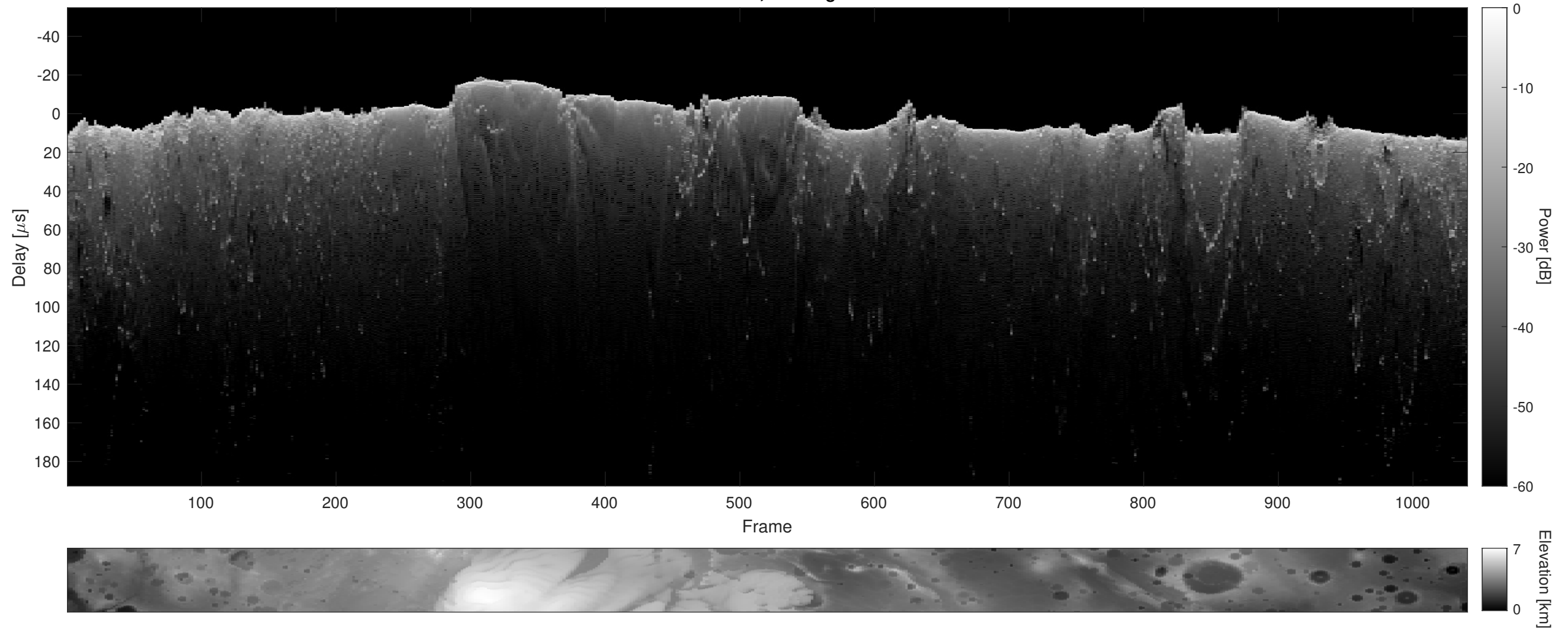
Orbit 10713, Cluttergram
