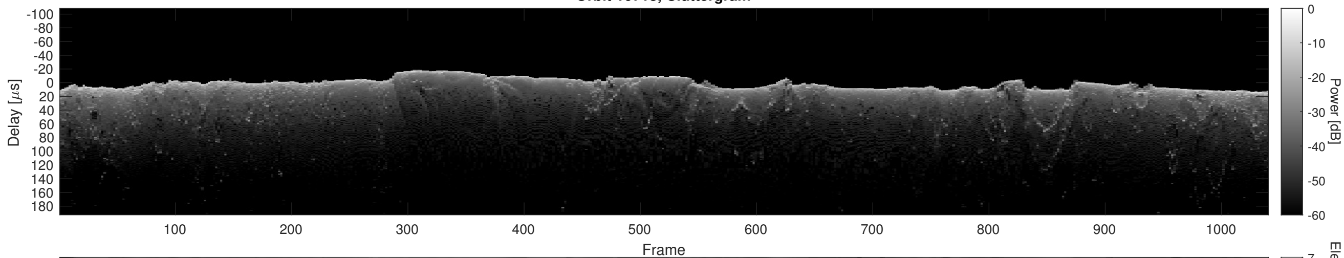
Orbit 10713, Cluttergram
