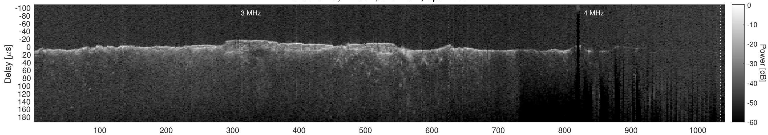
Orbit 10713, Cluttergram
