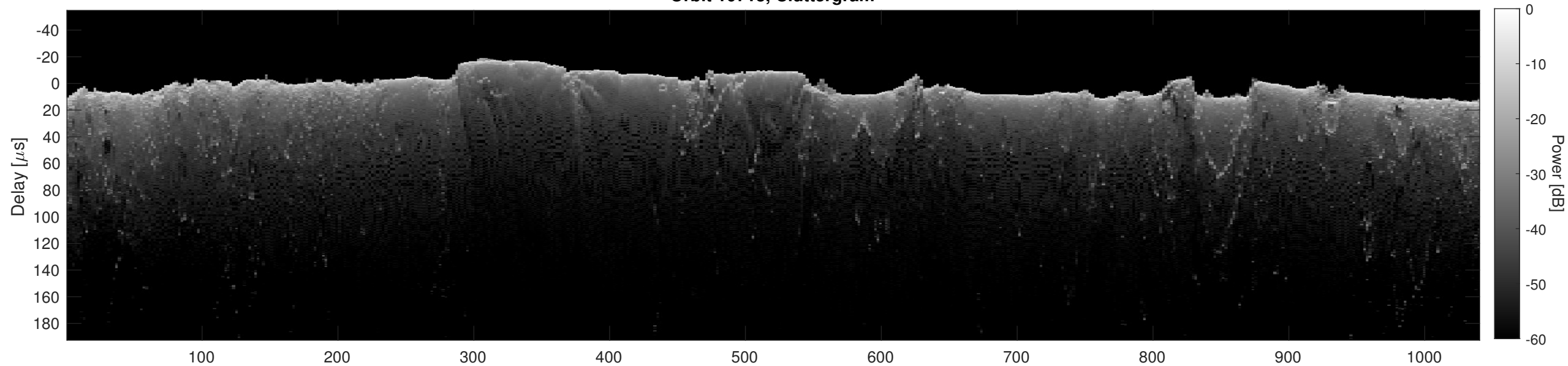
Orbit 10713, Cluttergram
