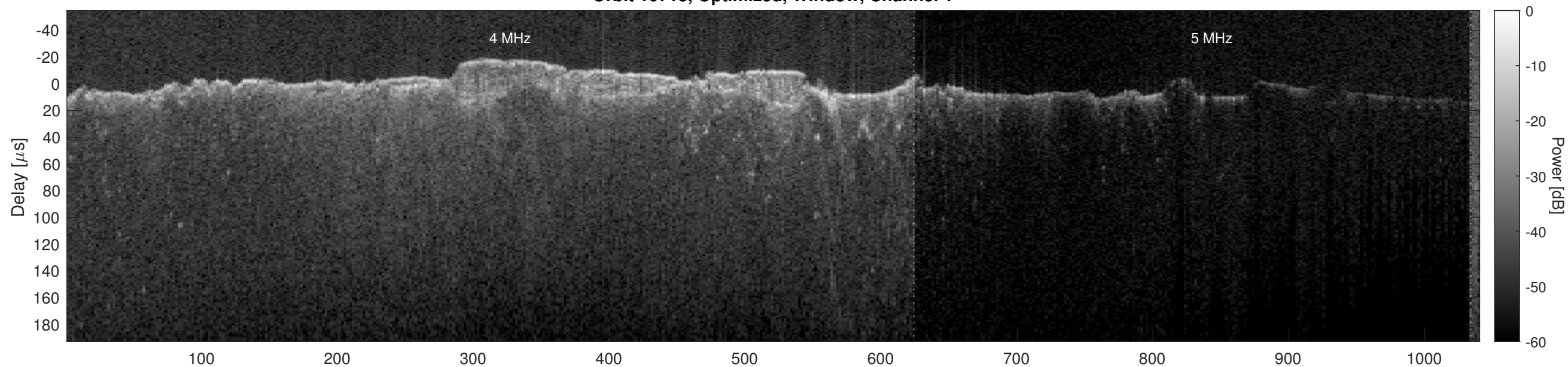
Orbit 10713, Optimized, Window, Channel 2
