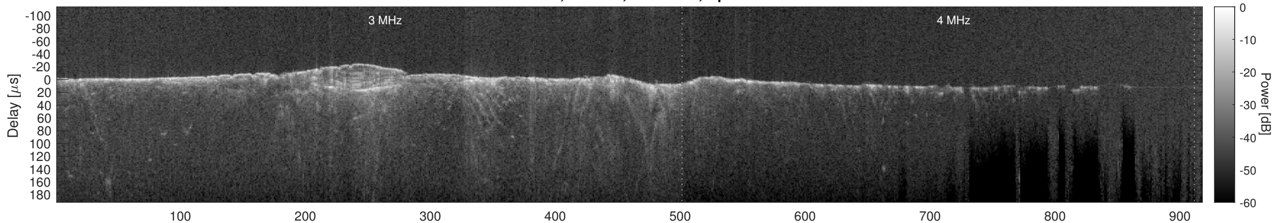
Orbit 10714, Cluttergram
