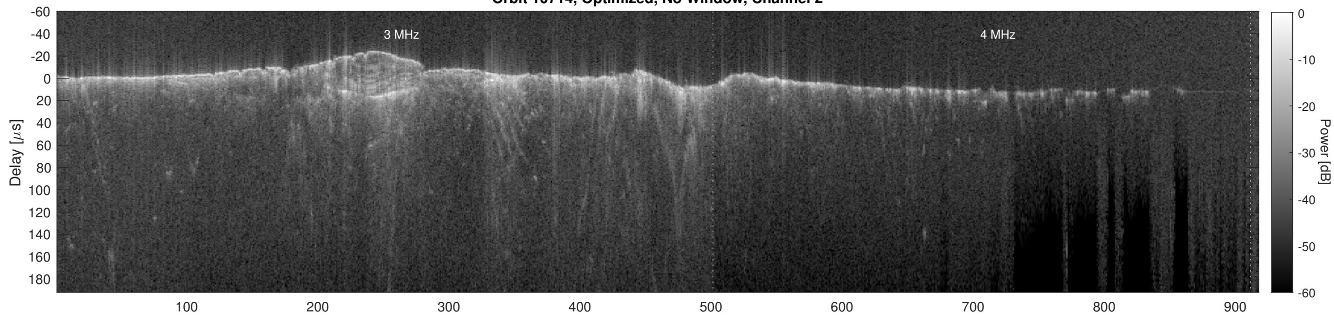
Orbit 10714, Cluttergram
